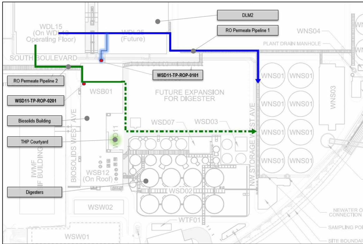
Figure P4F. 2 Indicative location of ROP/G1 tie-in points for connections
